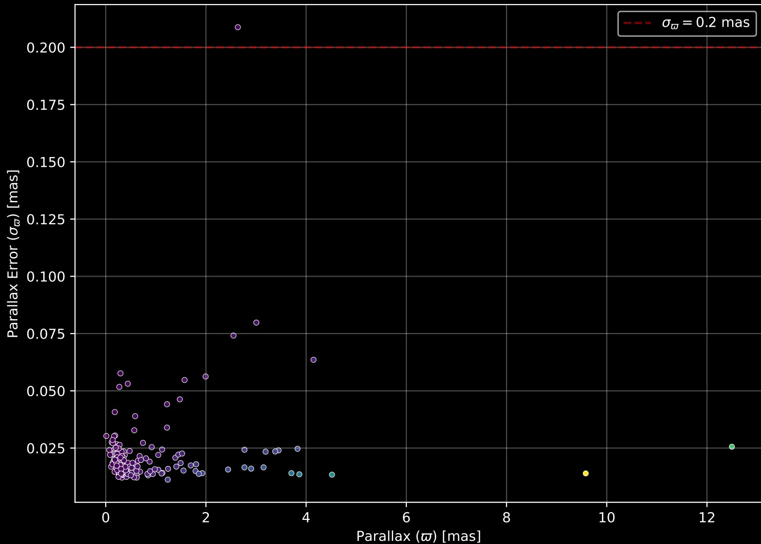
APOGEE DR17 Field: [158+12] Parallax Quality (n= 174)
