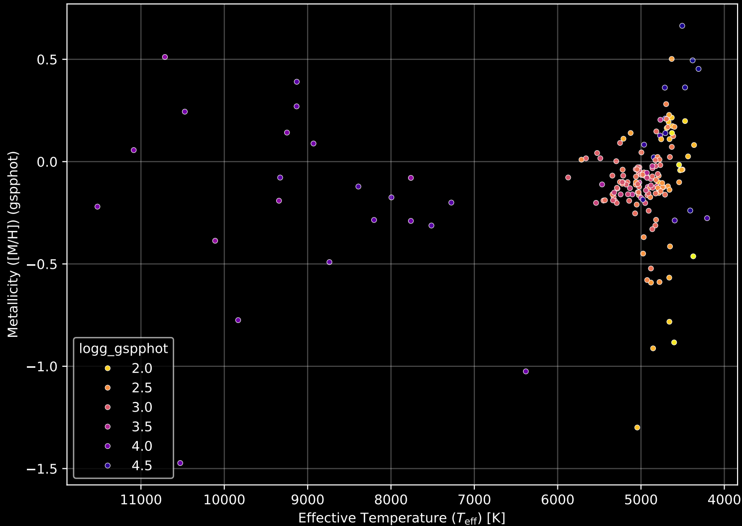
APOGEE DR17 Field: [158+12] Stellar Population Parameters (n= 174)
