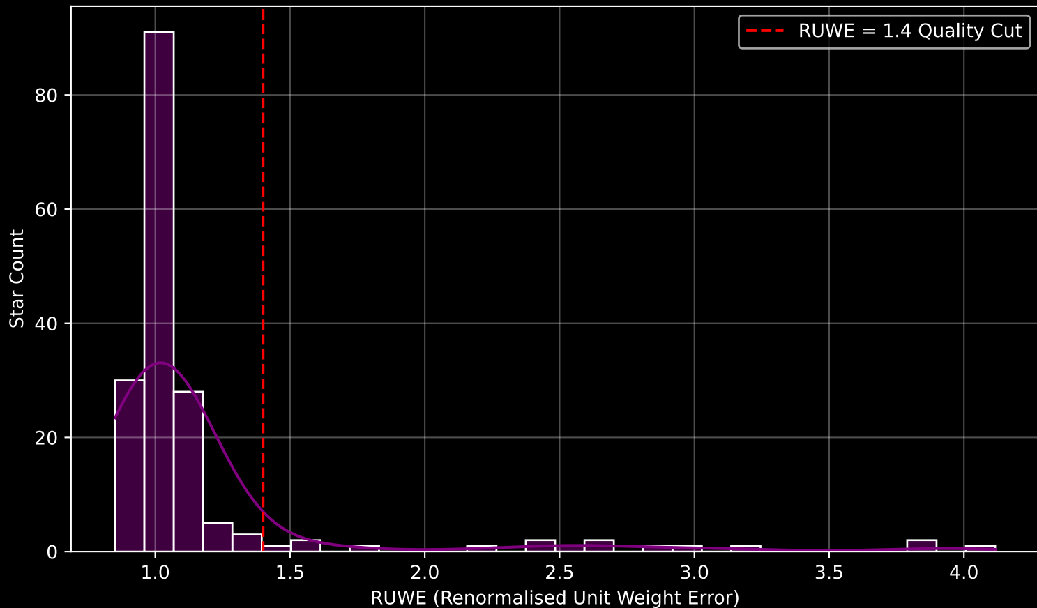
GAPOGEE DR17 Field [158+12] RUWE Distribution (n= 173)
