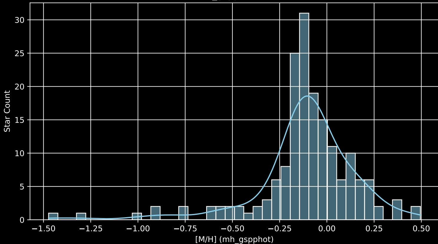
APOGEE DR17 Field: [158+12 [M/H] (mh_gspphot) (n= 171)
