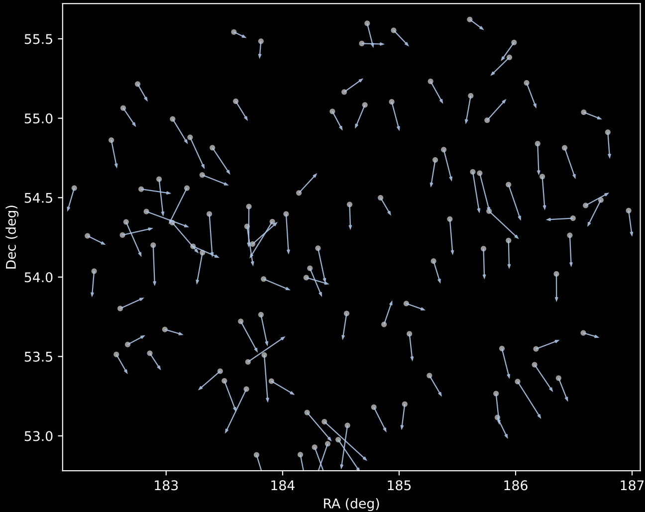
APOGEE DR17 Cluster 1 Proper Motion Vectors (n=107)
