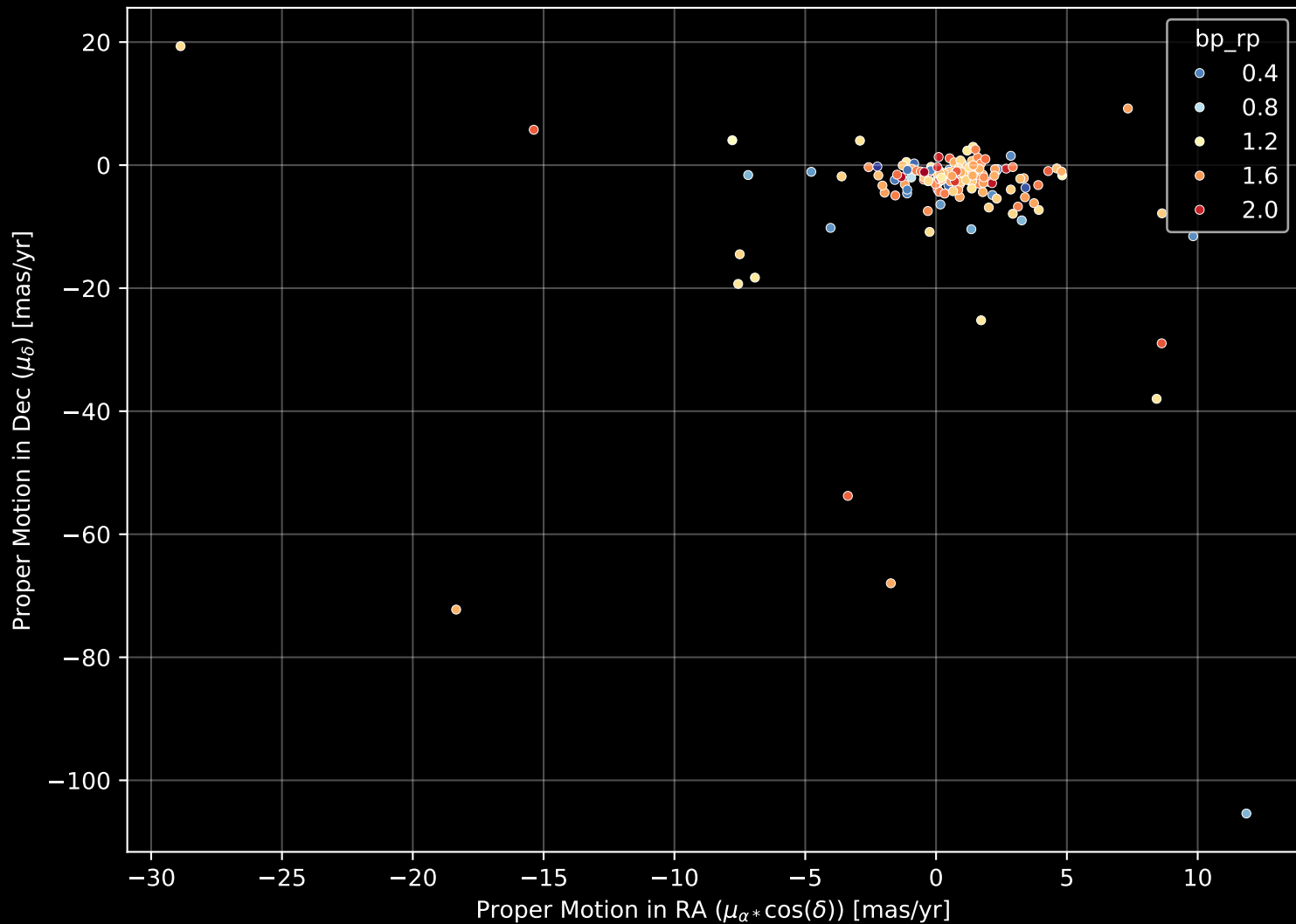
APOGEE DR17 Field: [158+12] Proper Motion Diagram (n= 174)
