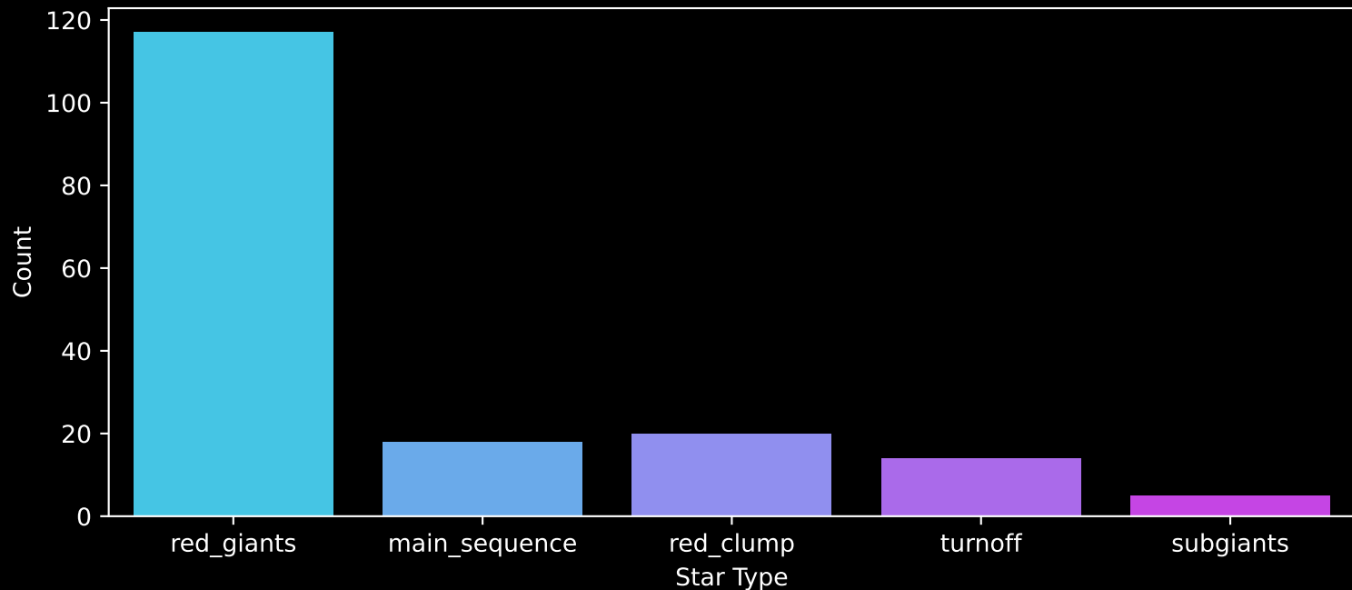
APOGEE DR17 Field: [158+12] Count plot of Star Type
